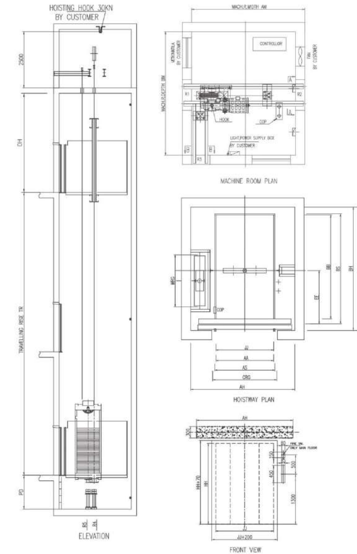
INACHI ELEVATOR Shaft and machine room dimensions for mini MR freight Elevator (single-door)
