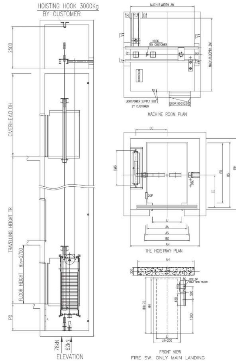
INACHI ELEVATOR Mini MR bed elevator (center opening)
