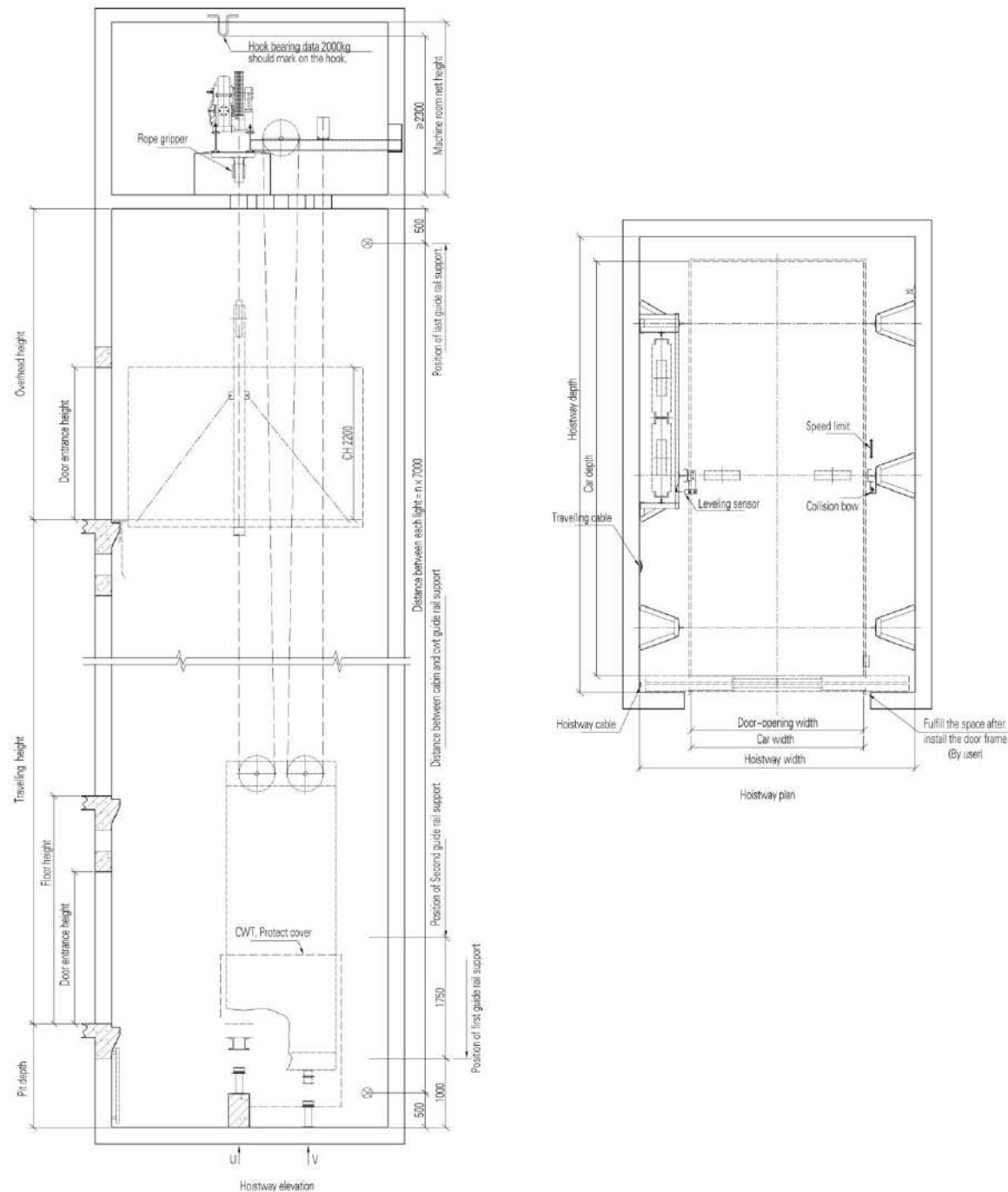
INACHI ELEVATOR Car elevator construction parameters
