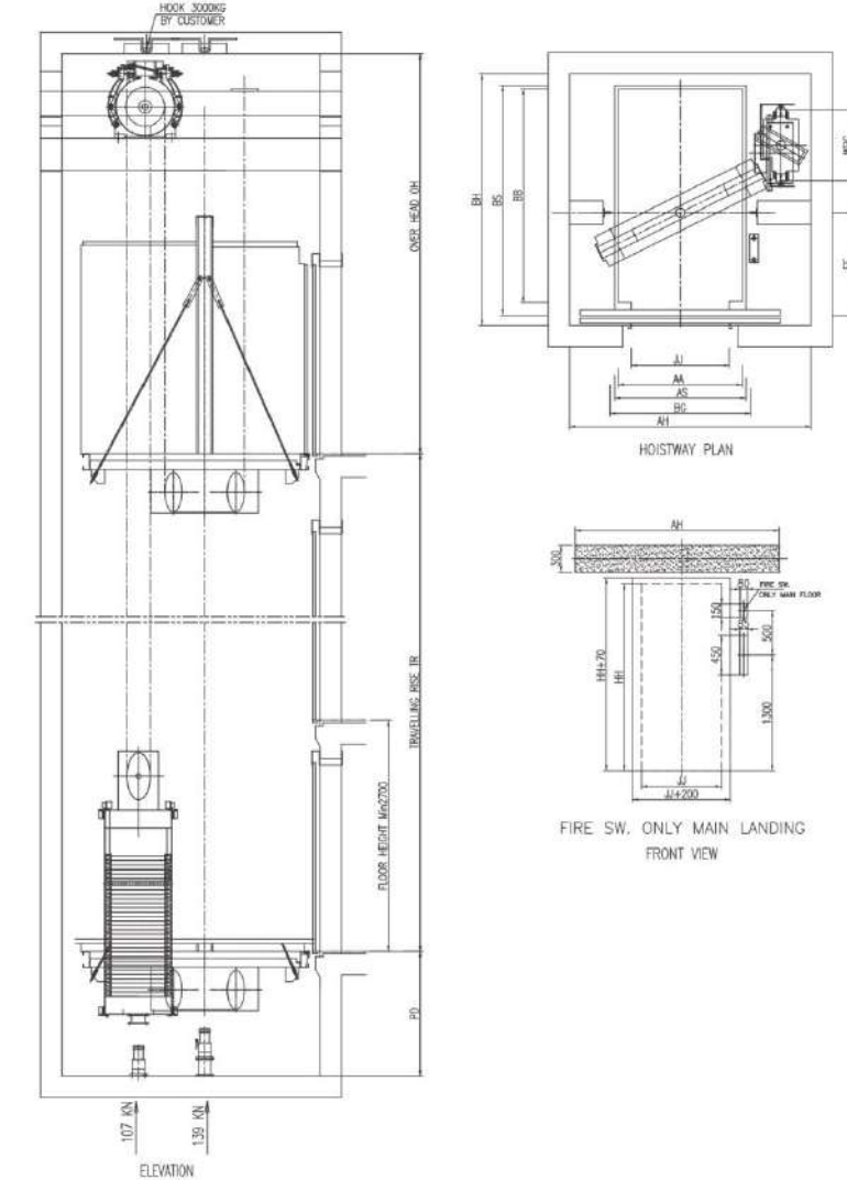
INACHI ELEVATOR Machine room less dimensions in the hoistway for bed elevator (CO)
