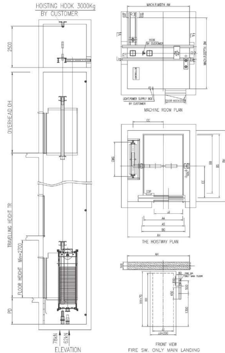
INACHI ELEVATOR Mini MR bed elevator (side opening)
