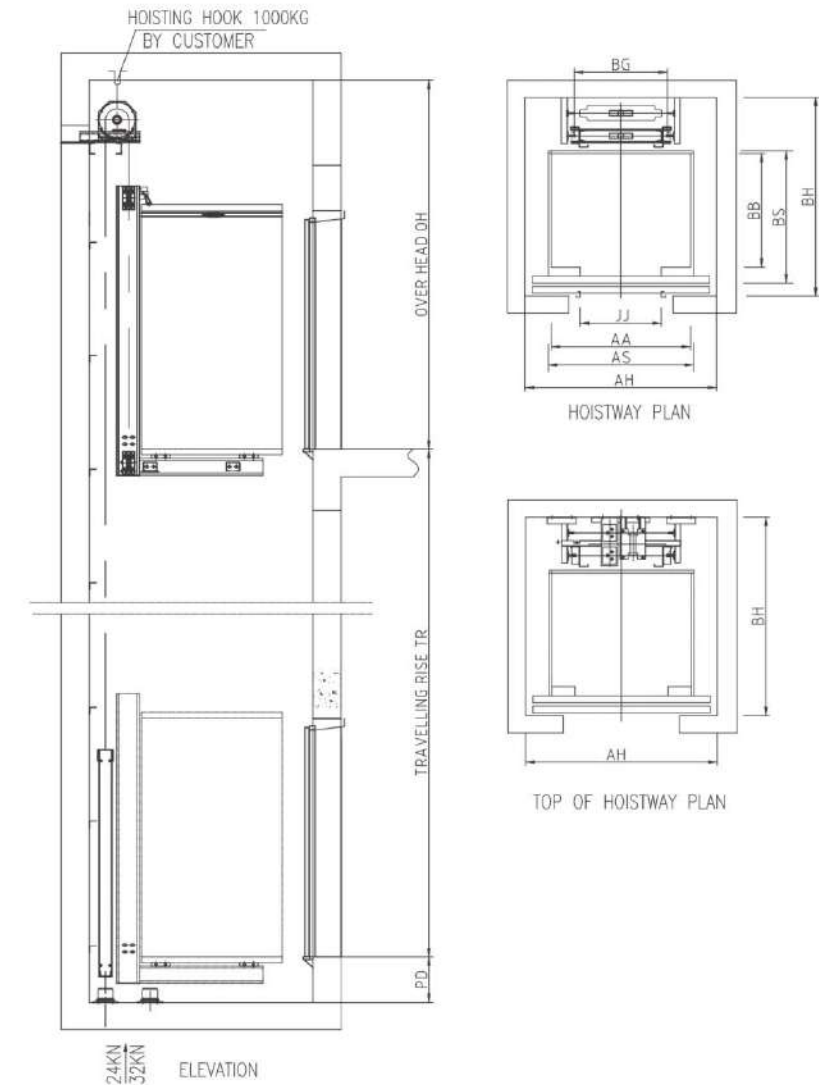
INACHI ELEVATOR home elevator (counter-weight on rear side)
