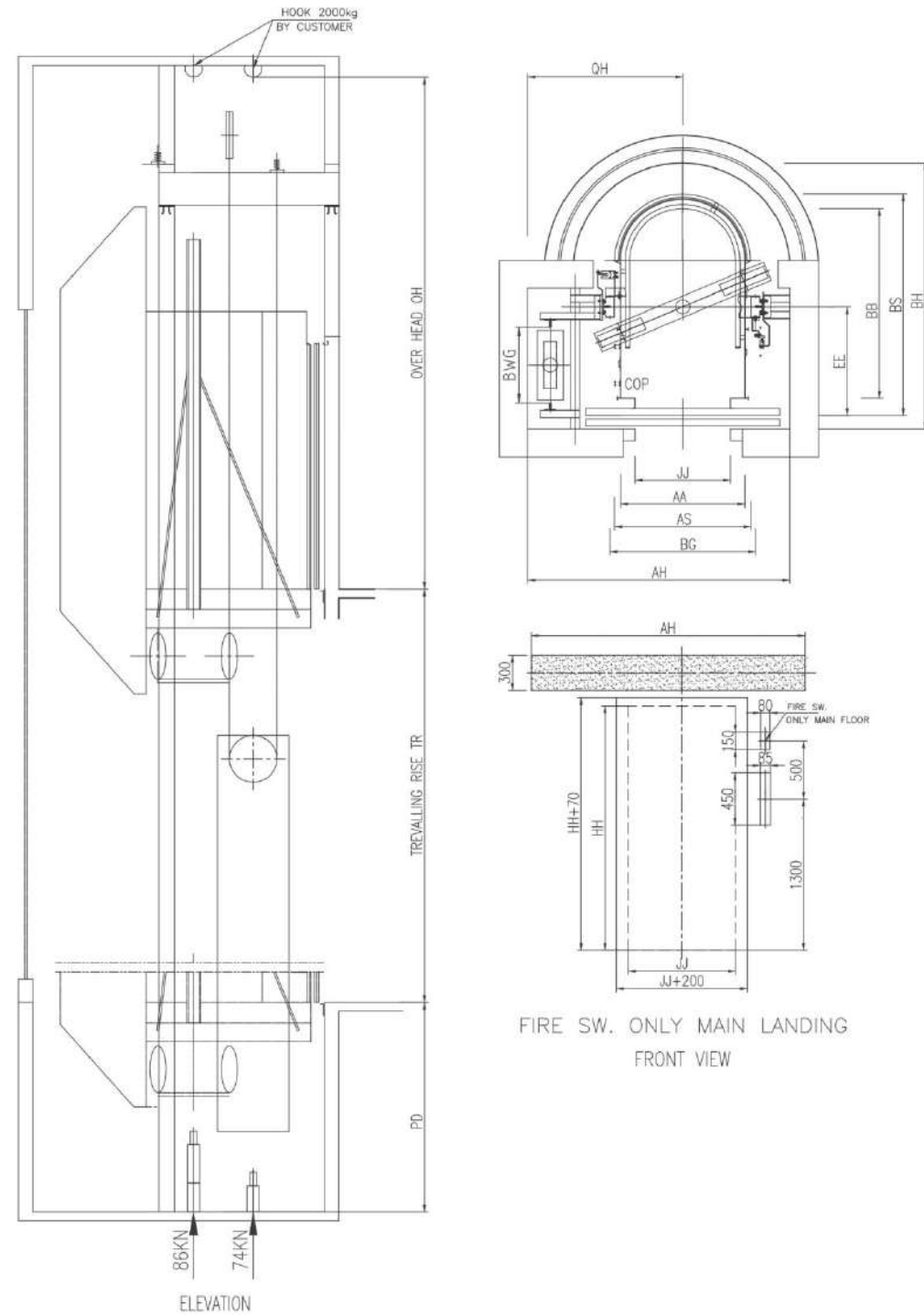
INACHI ELEVATOR panorama elevator (semi-cicle)
