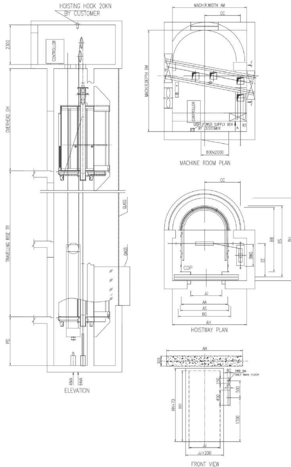
INACHI ELEVATOR panorama elevator (semi-circle)
