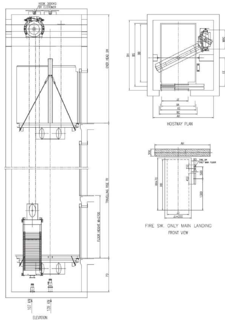
INACHI ELEVATOR Machine room dimensions in the hoistway for bed elevator (side opening)
