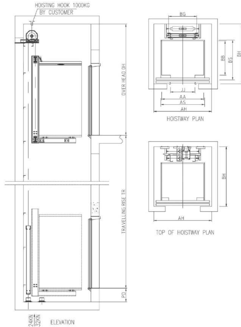
INACHI ELEVATOR home elevator (counter-weight on one side)
